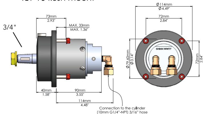
TL1-16 flush mount
