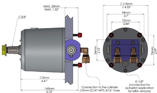
Pump:TL2-30 MRA Front mounting
